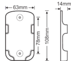
Remote holder
