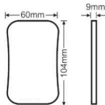
RF remote
